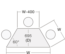
Trapezoidal: W x D x H
