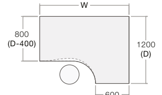
Crescent: W \times D \times H Available on Kassini, Optima Plus, Callisto, Windsor and Flexi
